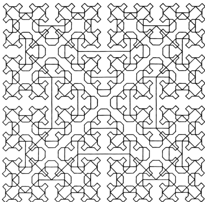
Figure 1.1 Sierpinski Curve
