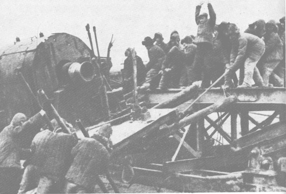
In the early period of building the Tachang Oilfield, Wang Chin-hsi and his 1205 Drilling Team, in the spirit of self-reliance and hard struggle, carrying and dragging the drilling rig to the well site to be installed.
