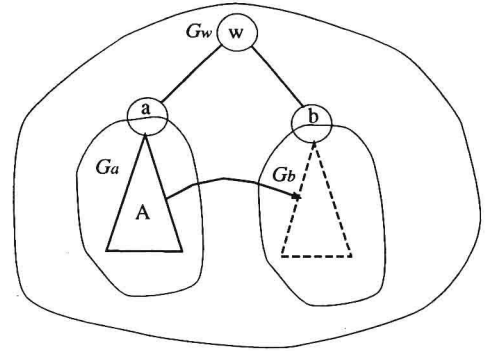
Figure 3: Moving a sub-structure A from one enclosing group to another.
