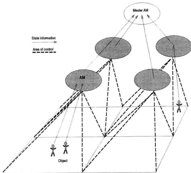
Figure 1: (Aura manager hierarchy)
