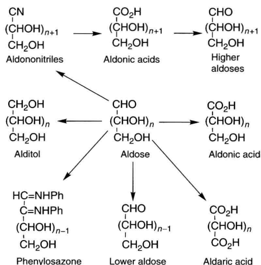
Scheme 1 Major transformations of aldoses.
