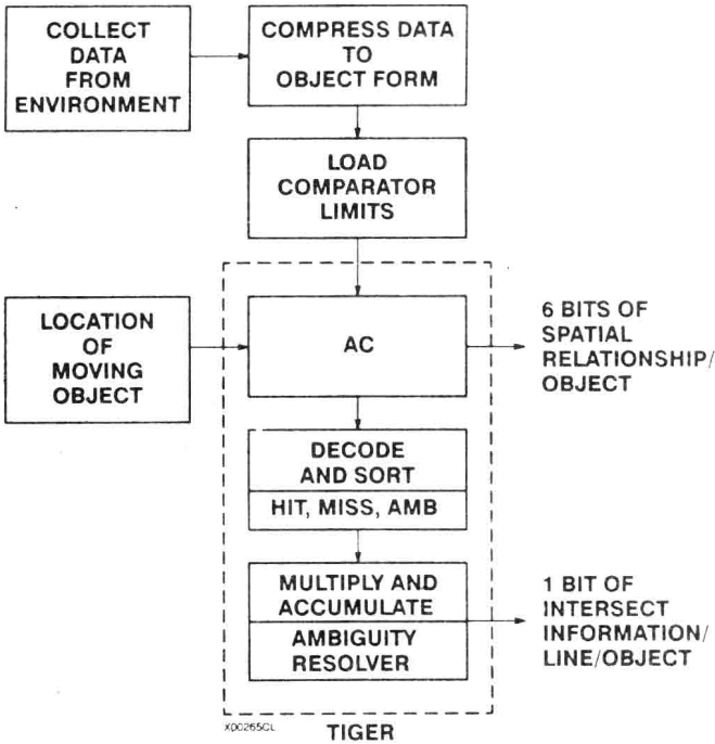
Fig. 2. Data flow using TIGER hardware.
