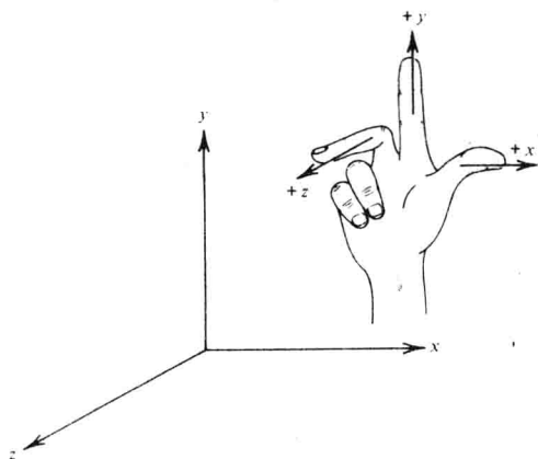
Figure 1-1 A right-hand coordinate system.
