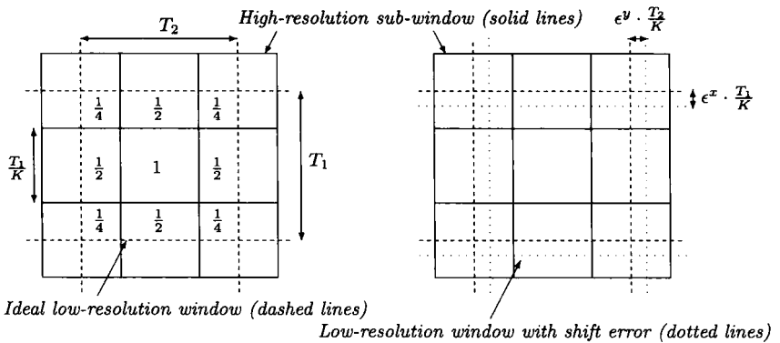
Figure 1.1 Windows without and with shift error when K = 2 (left and right respectively).
