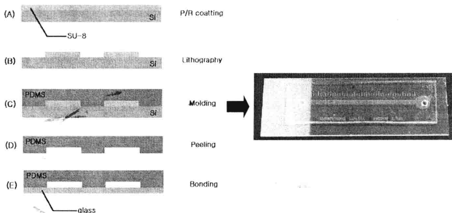
Fig. 4. Fabrication process and final module
