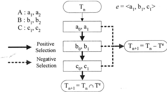
Fig. 1. Training process of DNA based version space learning for an example \langle a_1, b_1, c_1 \rangle
