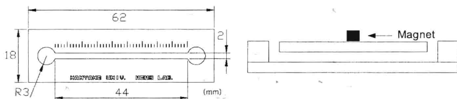
Fig. 3. Layout of the bead separation module. Top view (left) and side view (right)
