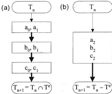
Fig. 2. Modified version of the learning process, which uses only positive selection for an example \langle a_1, b_1, c_1 \rangle . (a) is for a positive example, and (b) is for a negative example
