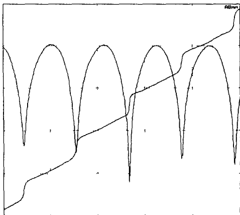
(Left) Transmission through a Michelson Interferometer at 285 GHz. Vertically: 10 dB and 360 degrees/div; horizontally: 0.47 mm/div.
