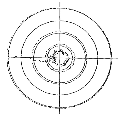
(Above) 94 GHz polar plot, 20 dB between solid circles. In series with a phase-shifter, attenuators at 10, 30, 50, 70 and 80 dB (inner, less regular circle).
