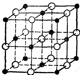
●Na + ○Cl -
