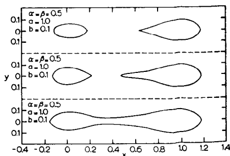
Fig. 9. Spot outlines at different cutoff values for an asymmetrical case. The range of phenomena that can be found is partially illustrated here. All the spots illustrated will, in practice, have a diffuse rather than a sharp boundary.
