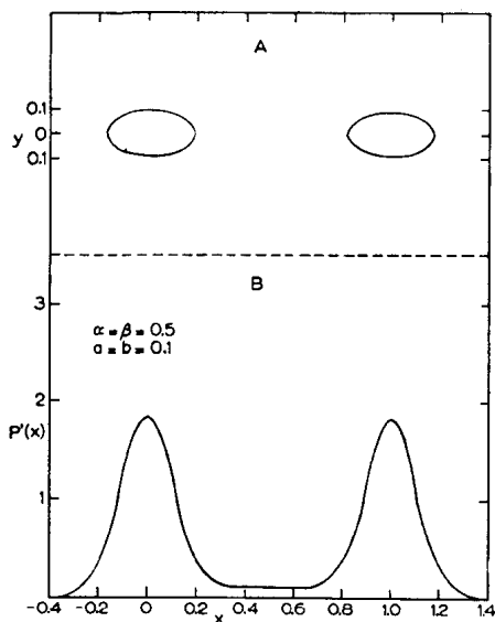
Fig. 2. Concentration profile and spot outlines for a symmetrical case. With a more sensitive method of detection, a continuous streak would exist between the two spots corresponding to the finite concentration between them.
