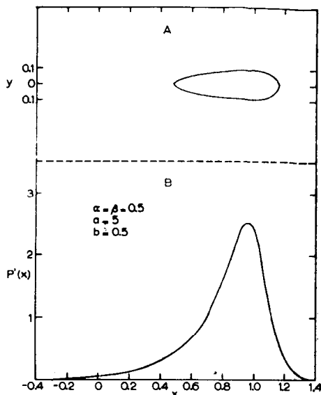
Fig. 7. Asymmetrical case in which one spot has essentially disappeared. Notice the extended tailing in the concentration profile and in the spot.
