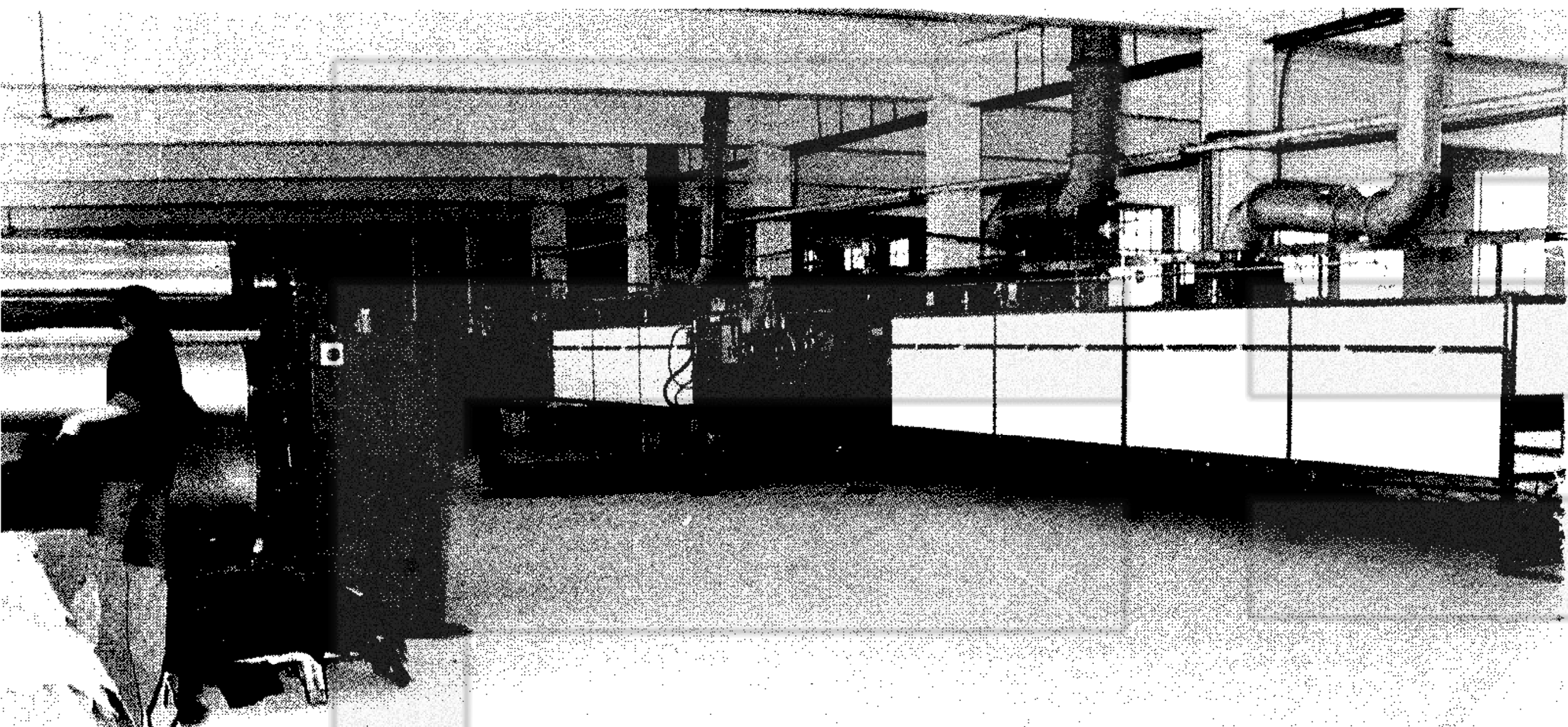
3. 整饰牛斜面革生产线 A conveyor-belt that trims and decorates cowhide
