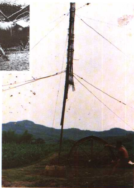
卓筒井小花车采卤
