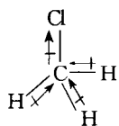
一氯甲烷 \mu = 6.21 \times 10^{-30} \text{C} \cdot \text{m}
