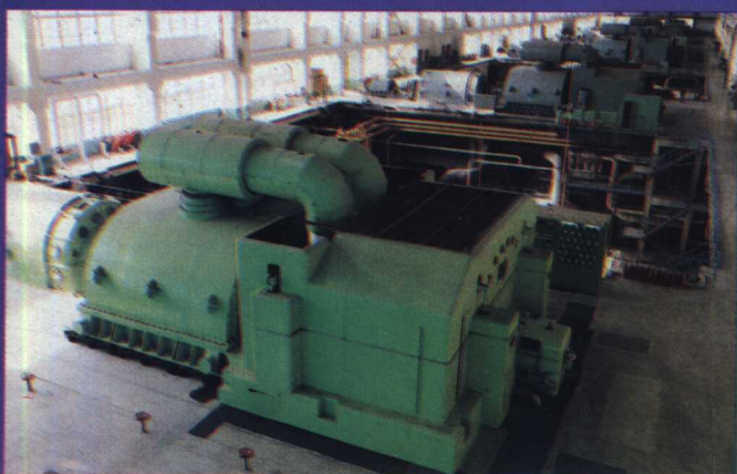
125MW中間再熱凝式汽輪發電機 125 MW REHEAT CONDENSING STEAM TURBINE-GENERATOR
