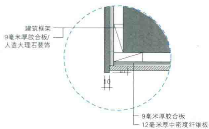
细节图B
