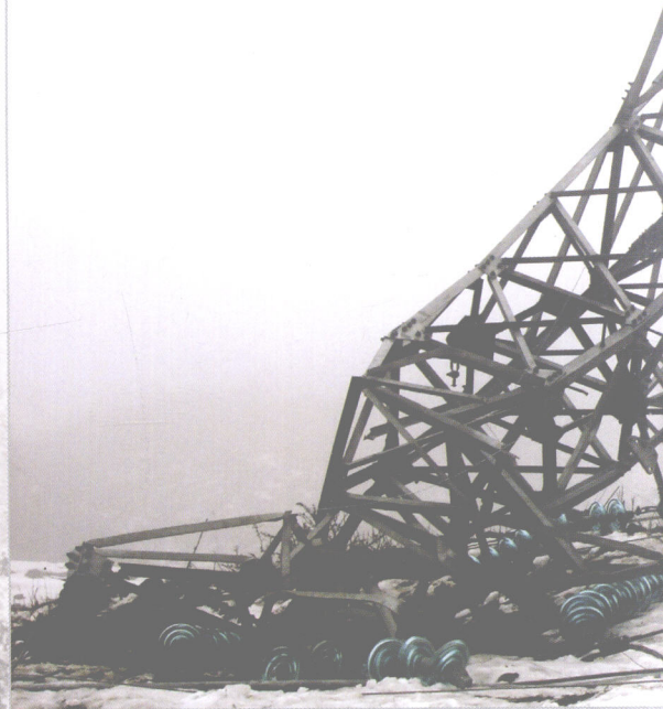
倒塌的110千伏镇威线 110 kV Zhenwei power transmission line.
