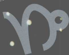
Capricorn
