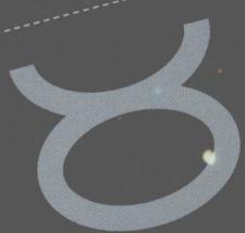
Taurus
