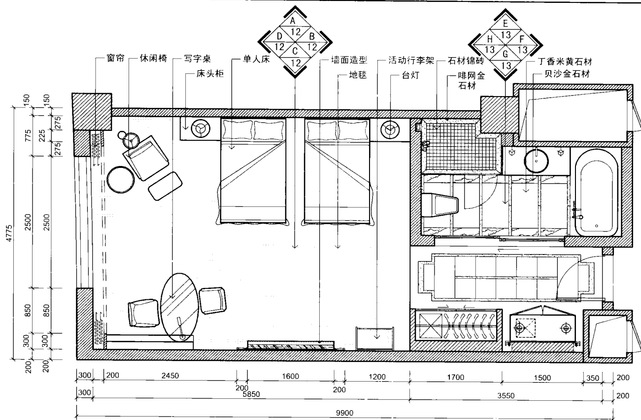
PLAN
