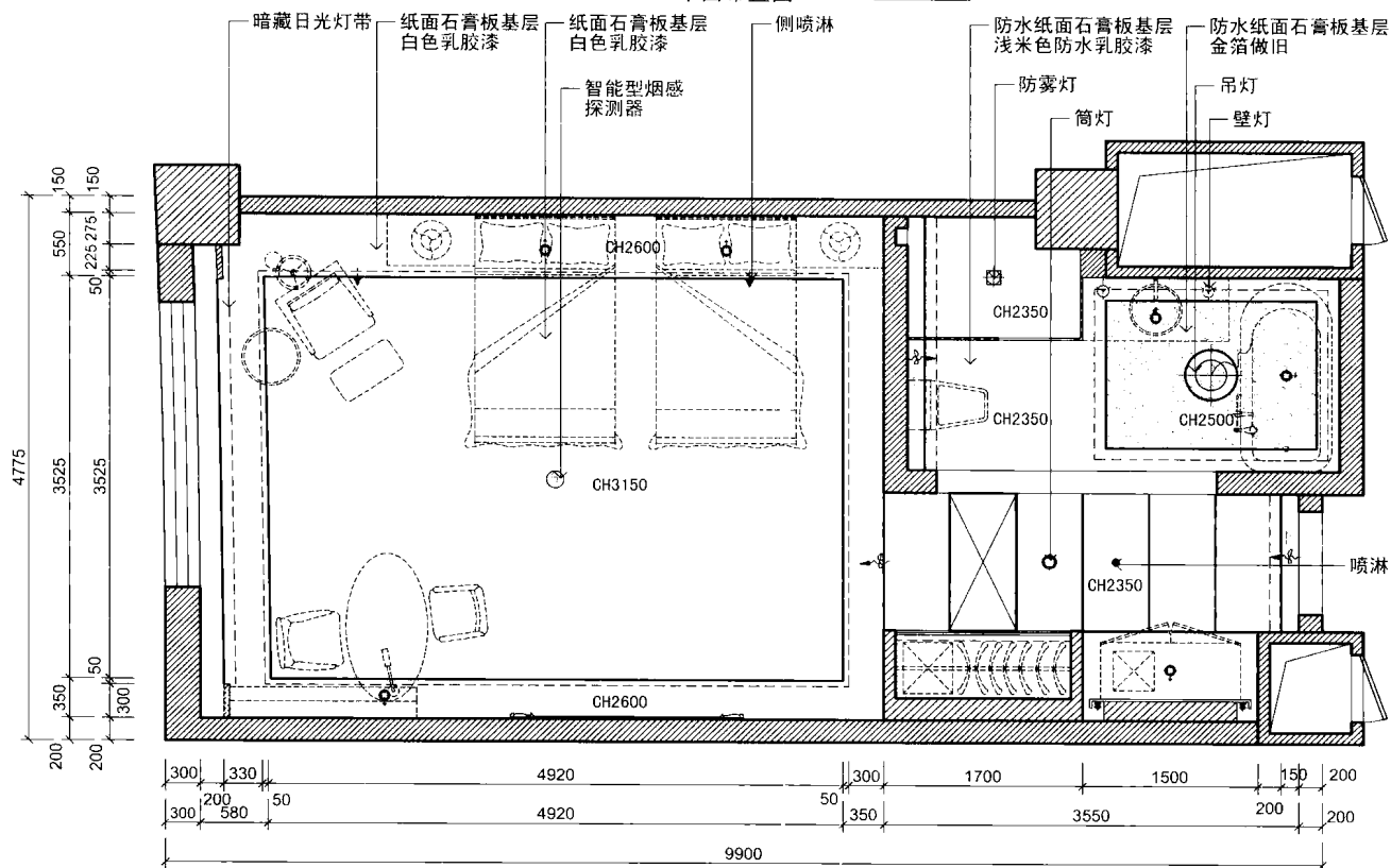
CEILING PLAN
