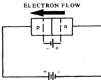
Fig. 1-6 With the bias of this polarity, the p-n junction offers low resistance and passes a heavy current
