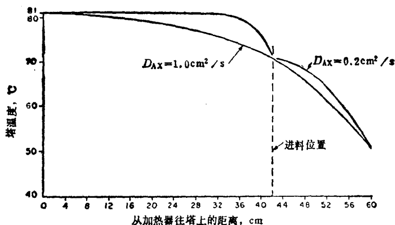
图 17-14 计算的塔-温度侧形[Moyers. et al. Am. Inst. Chem. Eng. J., 20, 1121 (1974).]
