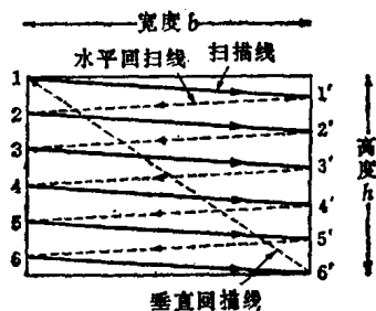
图1.6 逐行扫描
