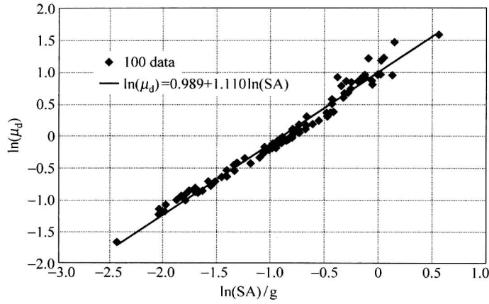
Fig. 8 Regression analysis of displacement ductility ratio versus spectral acceleration
