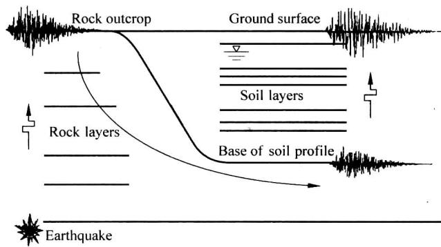
Fig. 4 Illustration of generating synthetic ground motion
