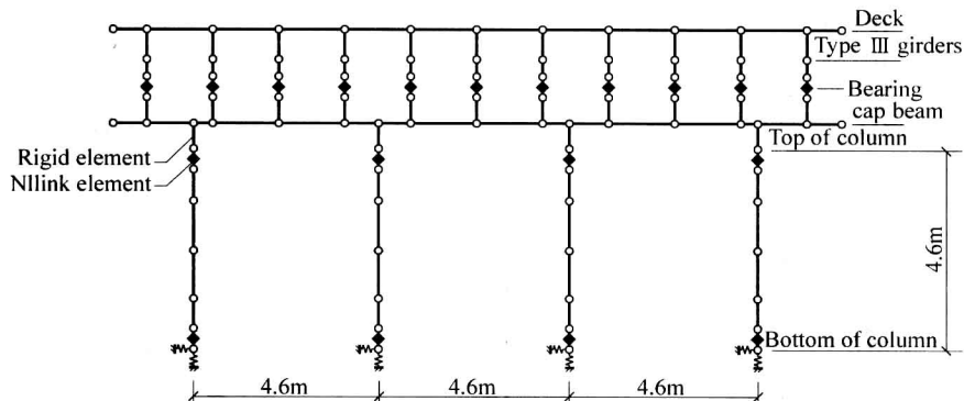
Fig. 3 Transverse view of the bridge finite element model
