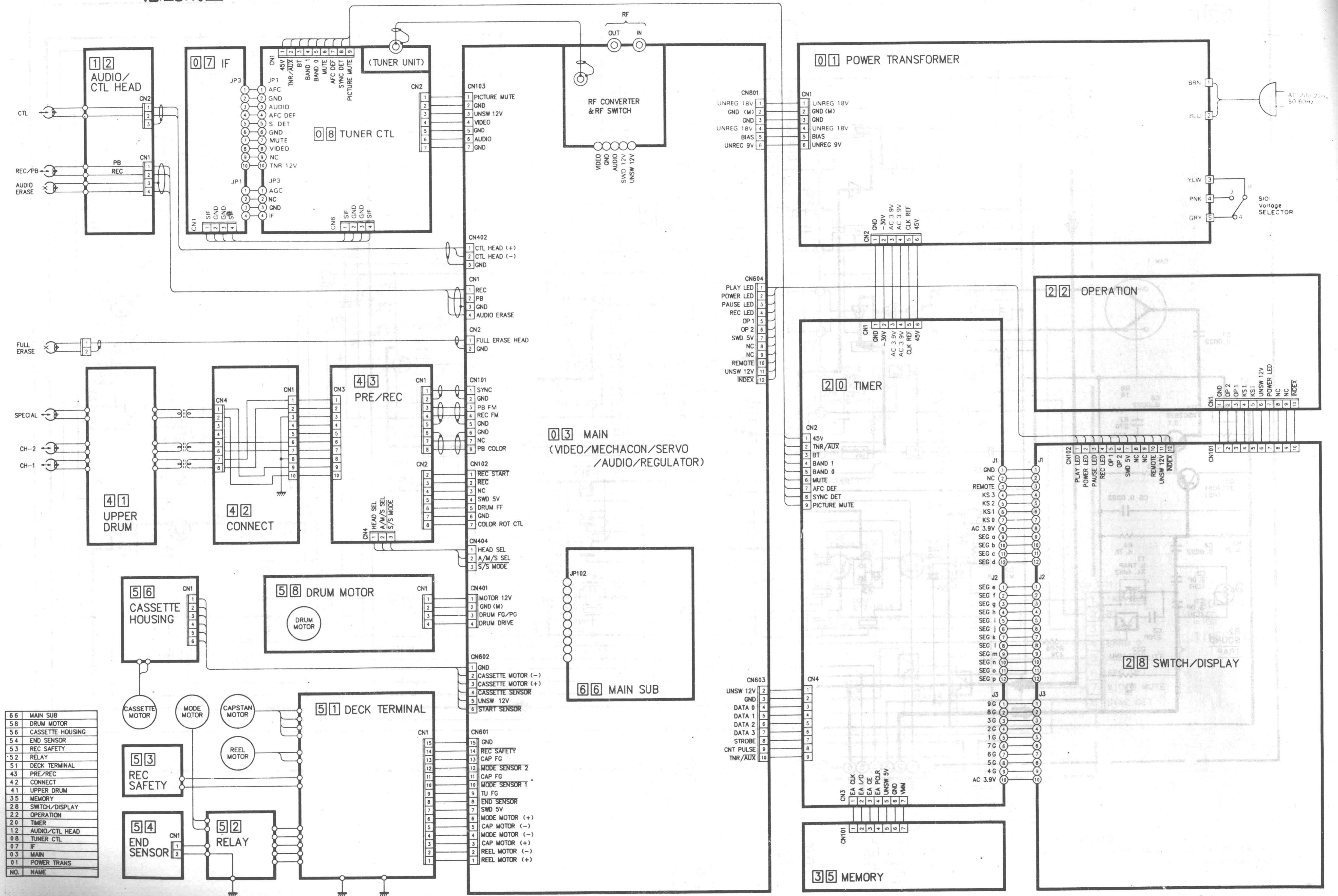
BOARD INTERCONNECTION DIAGRAM 总配线图
