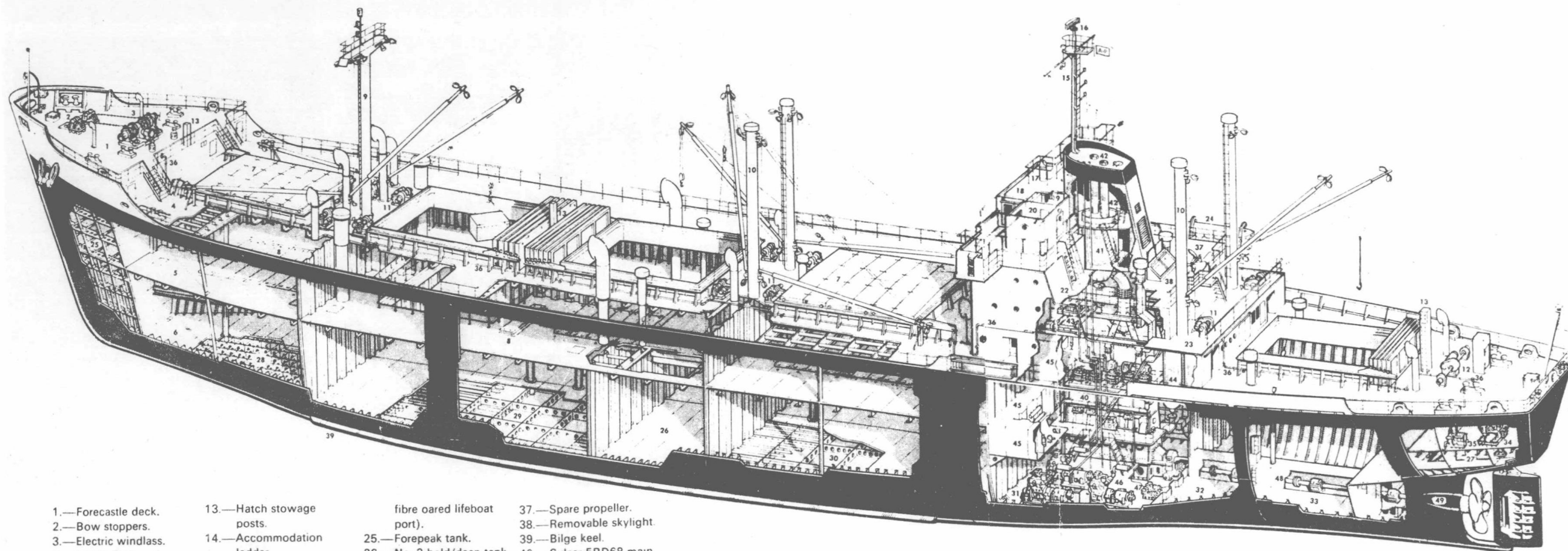
Cargo vessel.
