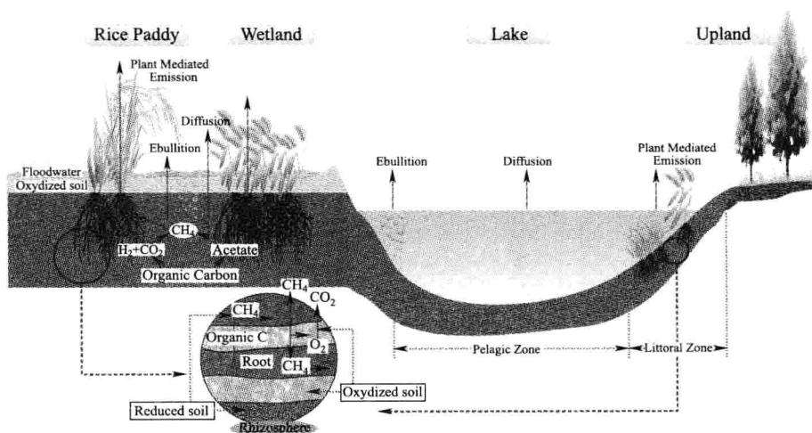
Fig. 1.1 A simplified illustration of \text{CH}_4 emissions from rice paddies, natural wetlands and lakes.
