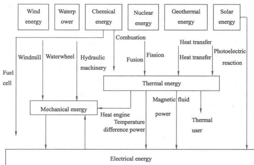
Fig. 1-1 Utilization of Thermal Energy
