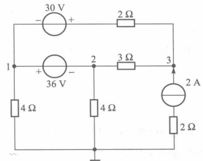
Figure 1.1.1 An example of node-voltage method
