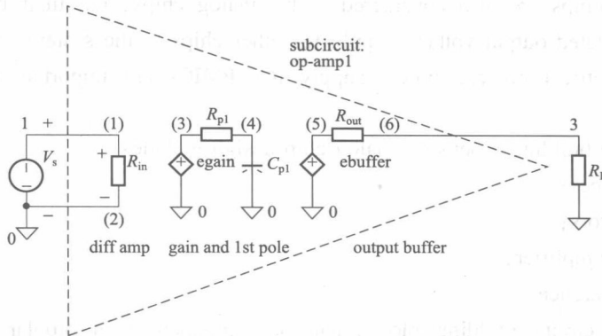
Figure 1.2.3 Basic operational amplifier (op-amp) model
