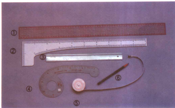
1. ①长直尺②L尺③短直尺④专用曲线尺⑤软尺⑥铅笔
