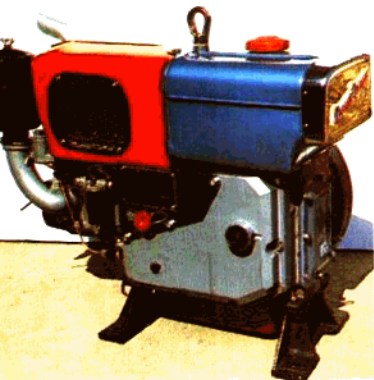
S 195 L 型柴油机 (冷凝式) Model S 195L Diesel Engine (condensation-type)
