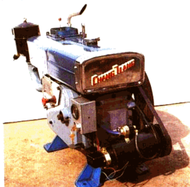
S 195 Q 型柴油机 (蒸发式、电起动) Model S 195Q Diesel Engine (ebullition-type, electric starting)
