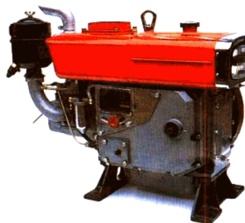
S195M型柴油机 (蒸发式、带灯) Model S 195 M Diesel Engine (ebullition-type, with lamp)
