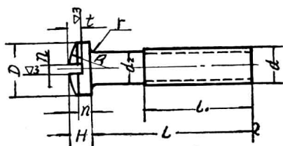
3. GB67-66 半园头螺钉
