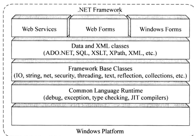
Figure 1 .NET Framework architecture
