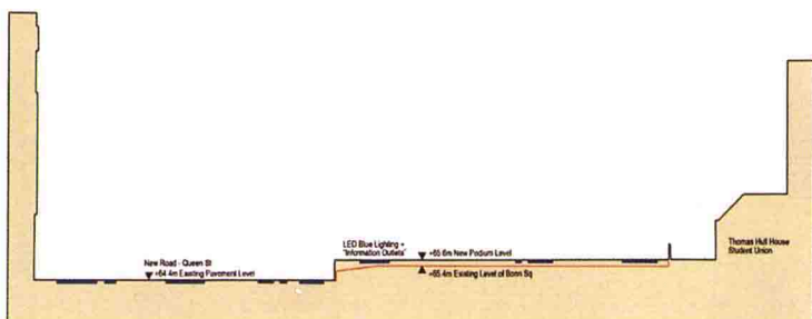
Section Profile of Bonn Sq (BB) Scale 1:200
