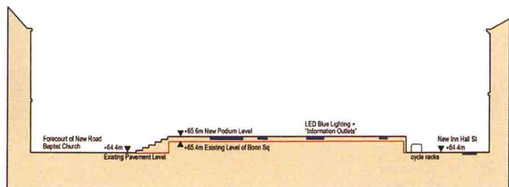
Section Profile of Bonn Sq (AA) Scale 1:200
