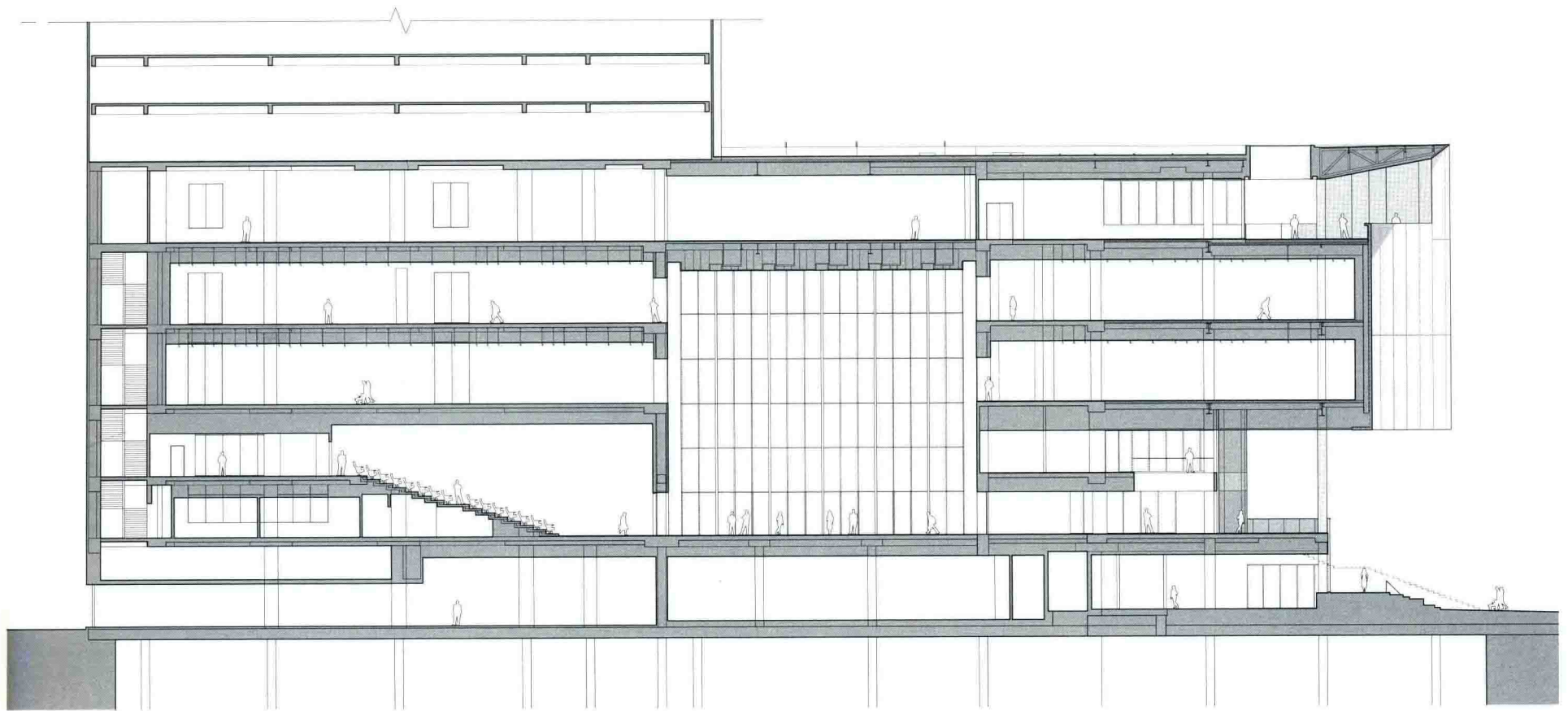
剖面图 -2 Sectional Drawing-2
