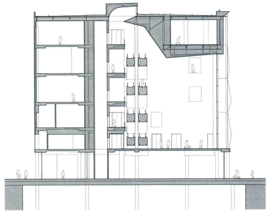
剖面图 -4 Sectional Drawing-4
