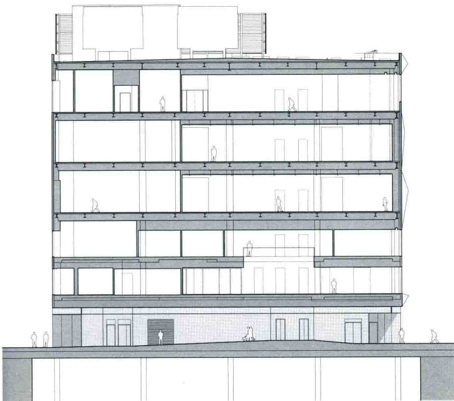
剖面图 -3 Sectional Drawing-3
