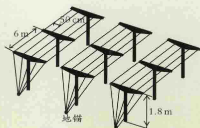
“T”形架
