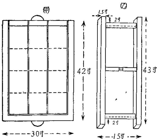
温床窗盖
