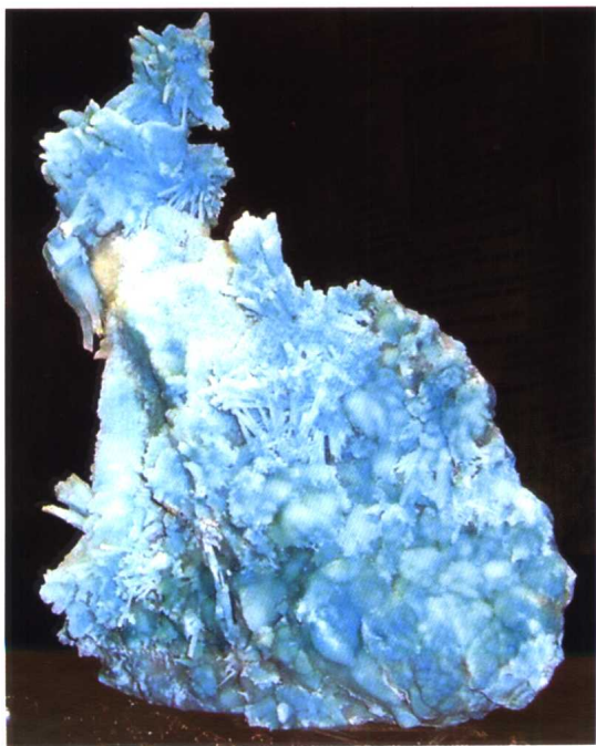
异极矿
