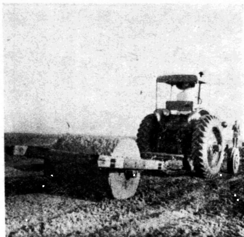
拖拉机压平大坝
