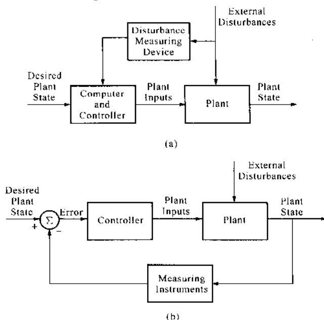
Fig. 2.1 Schematic representation
