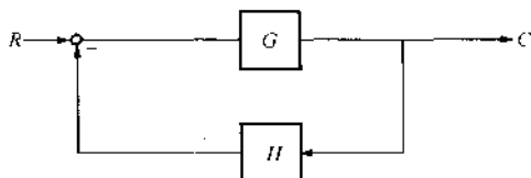
Fig. 2.3 Feedback system
