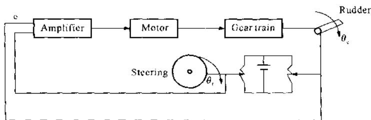
Fig. 1.4 Rudder control system
