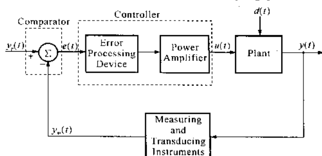
Fig. 2.2 Structure of single-loop feedback system
