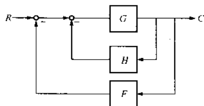
Fig. 2.4 Feedback system with two feedback loops
