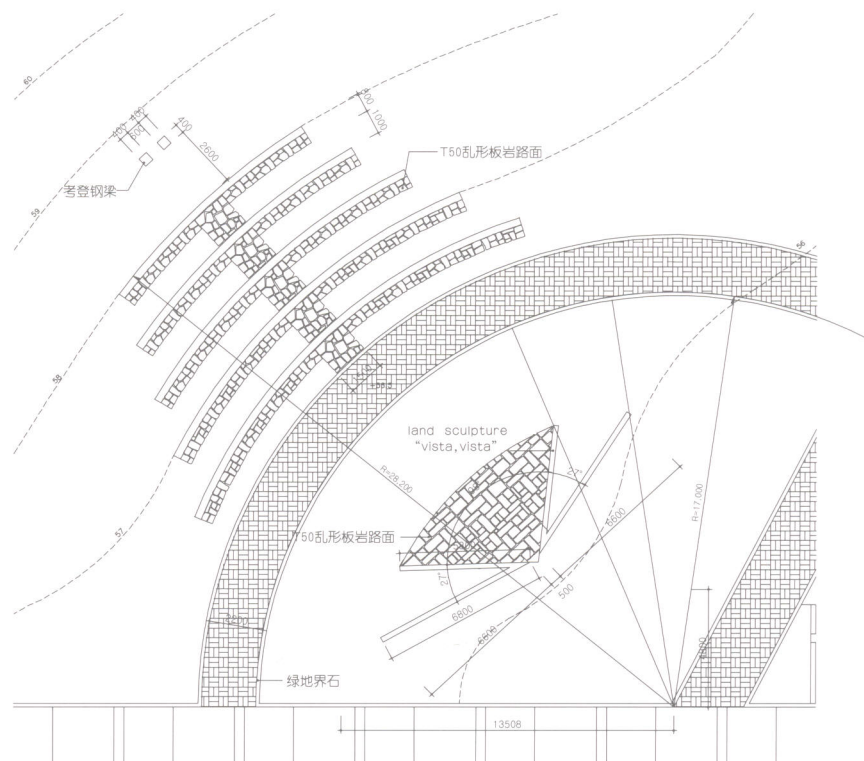
Outdoor stand - part plan
