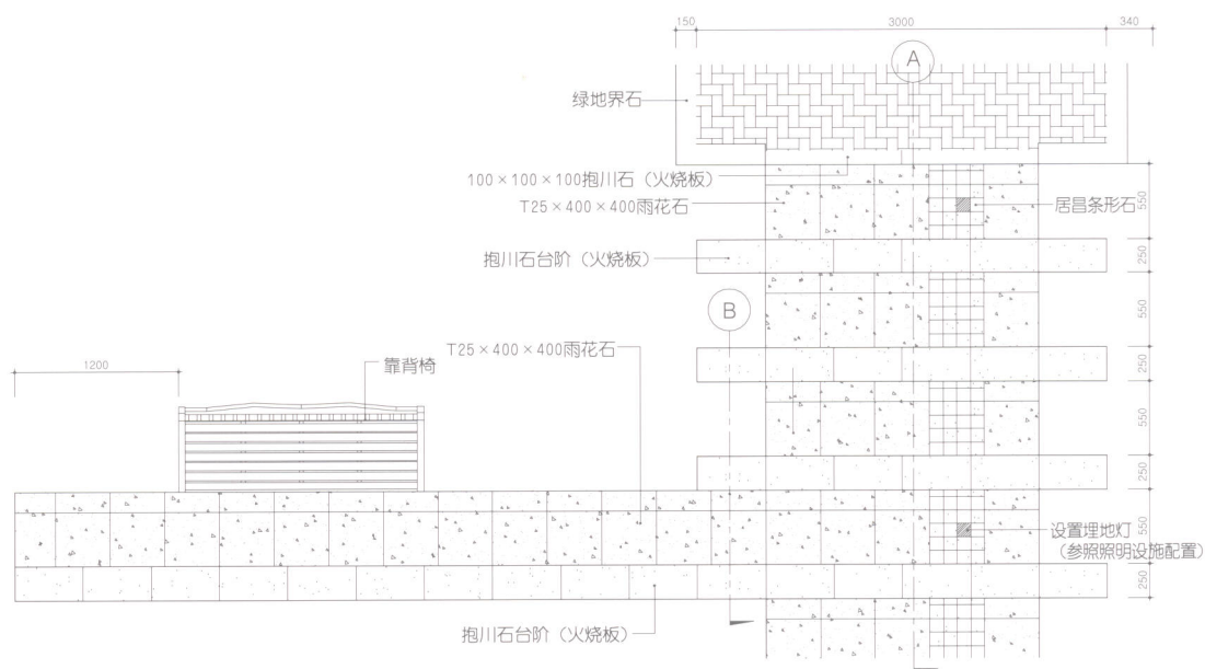
Stair garden stair - part plan
