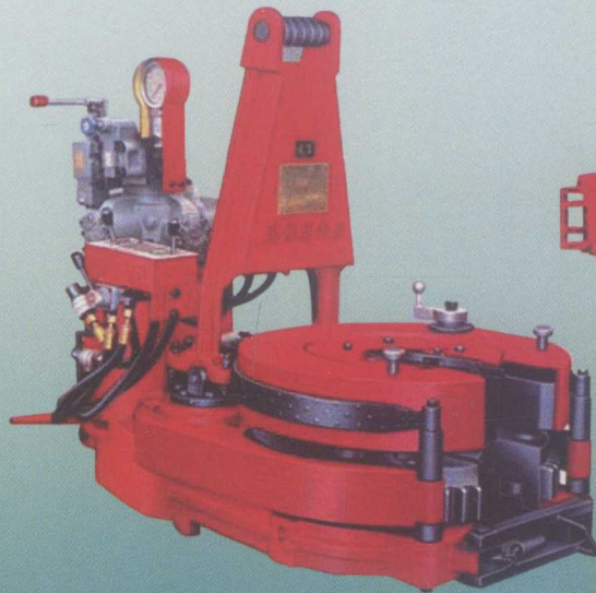
ZQ钻杆动力钳 Drill Pipe Power Tongs
