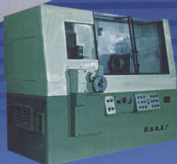
● S7620A内螺纹磨床
