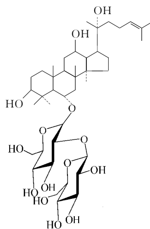
20(R)-人参皂苷 Rg 2
