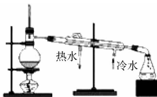
Figure 1.5 fractional distillation
