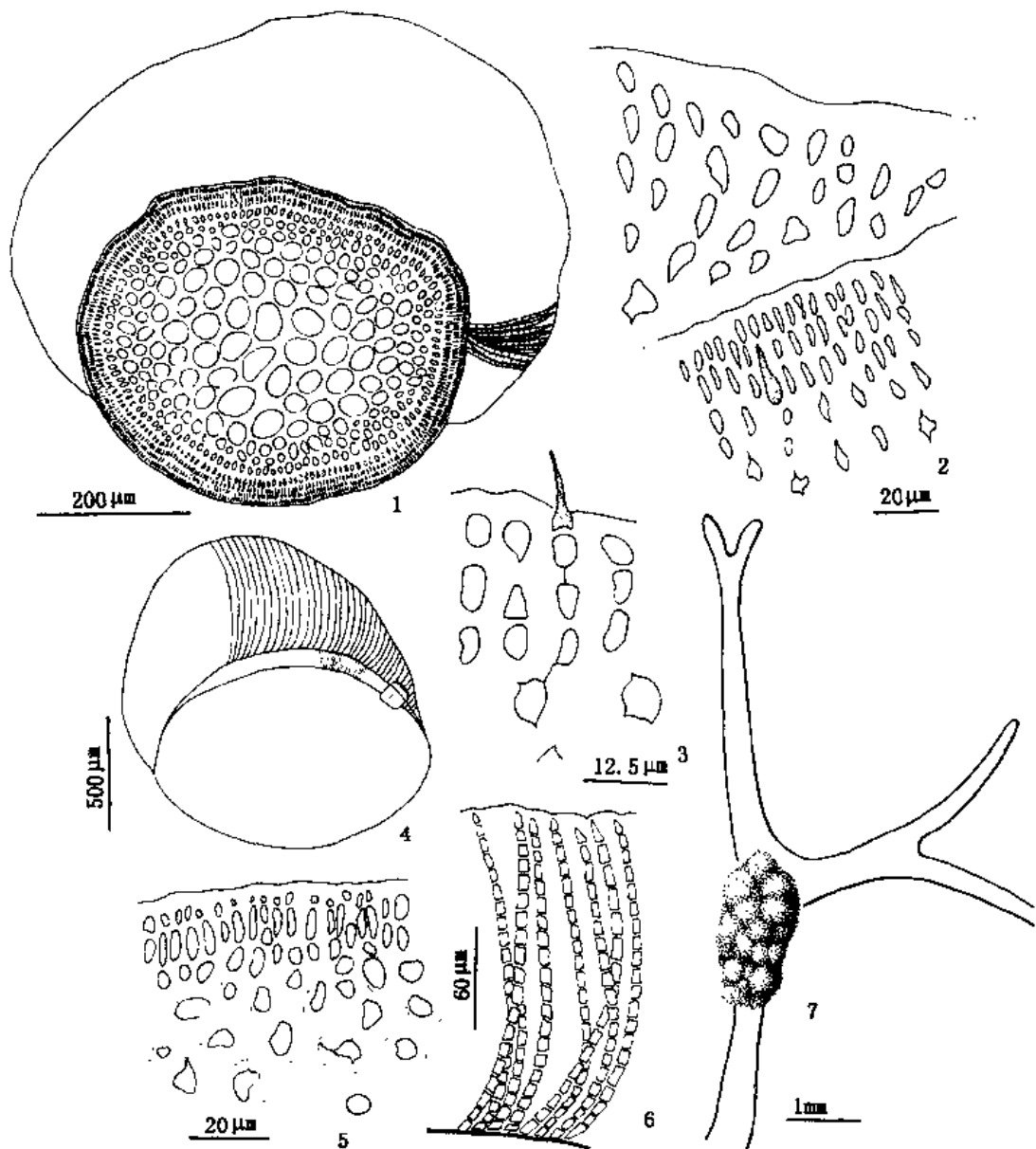
图2 莺歌海伊谷藻 Ahnfeltia yinggehaiensis Xia et Zhang 1. 藻体横切面 (AST 57—5799); 2. 轴的横切面, 示果胞 (AST 80—2331); 3. 果胞 (AST 80—2331); 4. 轴的横切面, 示辐射状的产孢丝 (AST 80—2331); 5. 精子囊窠切面观 (AST 80—2331); 6. 产孢丝放大图 (AST 57—5799); 7. 果孢子体外形图 (AST 57—5799)。 Fig. 2 Ahnfeltia yinggehaiensis Xia et Zhang 1. Transection of frond (AST 57—5799); 2. Transection of frond, showing carposogonium (AST 80—2331); 3. Carposogonium (AST 80—2331); 4. Transection of frond, showing radiating gonimoblast filaments (AST 80—2331); 5. Transection of spermatangia (AST 80—2331); 6. Enlargement of gonimoblast (AST 57—5799); 7. Carposporophyte (AST 57—5799).
