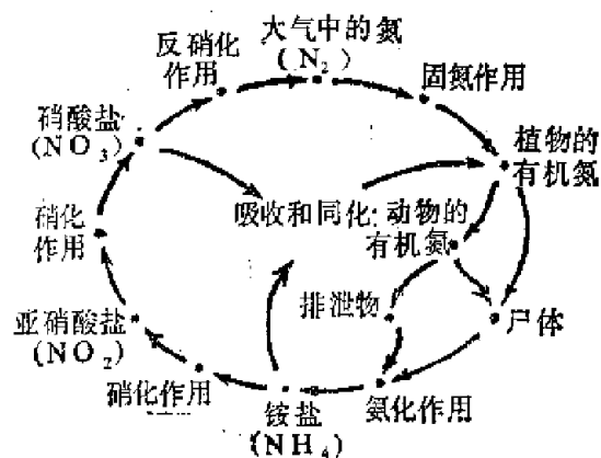
图绪-2 氮循环
