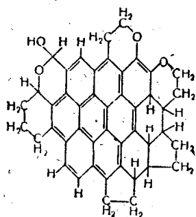
(III) C_{45}H_{34}O_8
