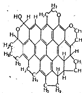
(VI) C_{46}H_{34}O_{11}
