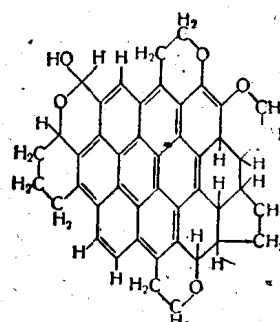
(V) C_{45}H_{34}O_8
