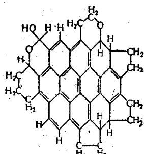
(VII) C_{45}H_{32}O_8
