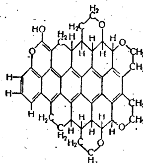
(IV) C_{45}H_{36}O_8
