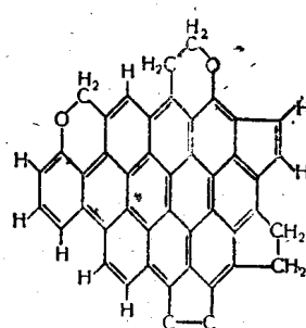
(IX) C_{45}H_{22}O_8
