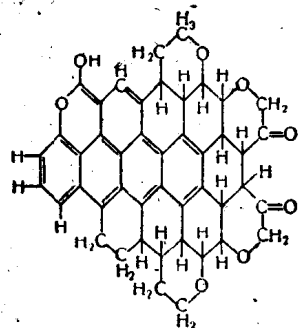
(I) C_{45}H_{34}O_8
