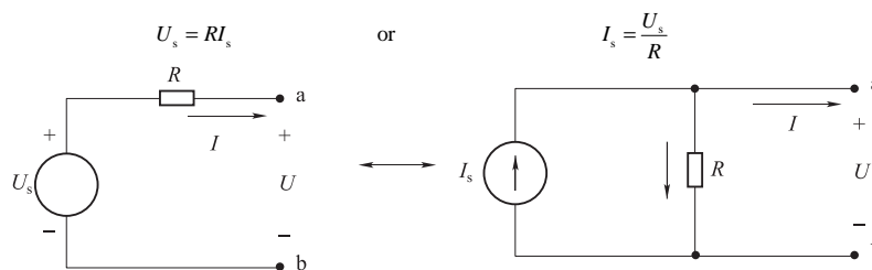
Fig.1.3 Source transformation
