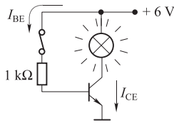
Fig.1.4 BJT used as an electronic switch
