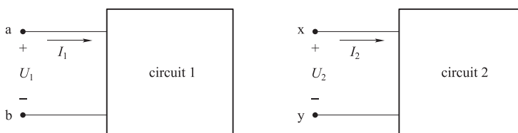
Fig.1.1 Circuit equivalence
