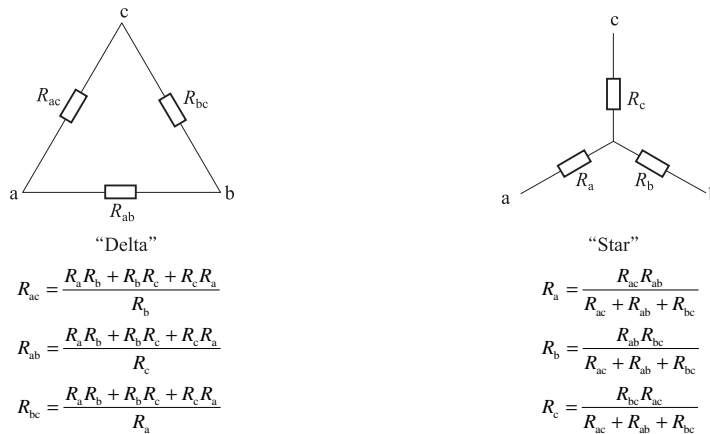
Fig.1.2 Star-to-delta transformation and Delta-to-star transformation
