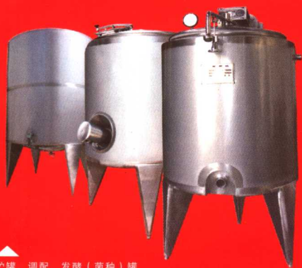
贮罐、调配、发酵(菌种)罐 Storage tank, Rearrangement pot, Fermentation(fungus)pot
