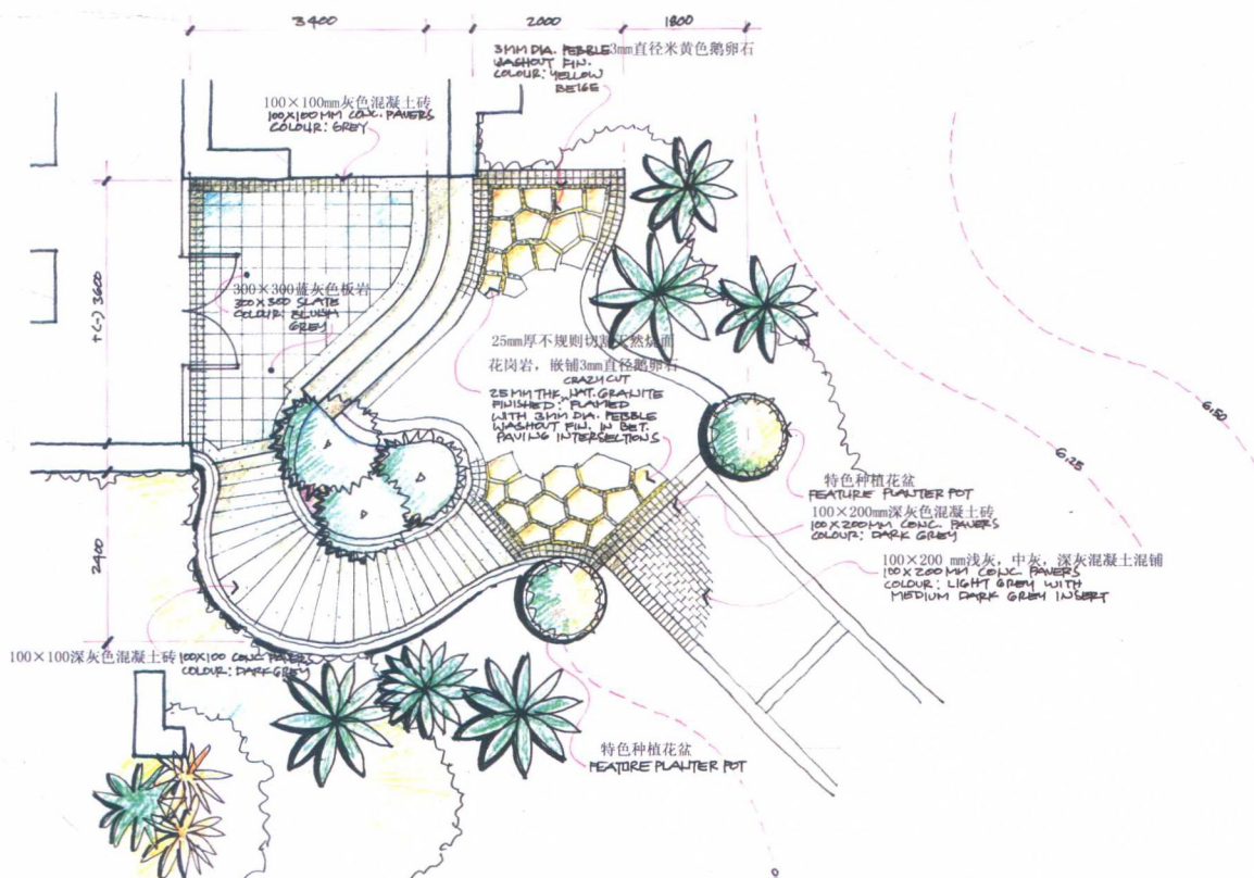
PART PLAN: BUILDING ENTRY
